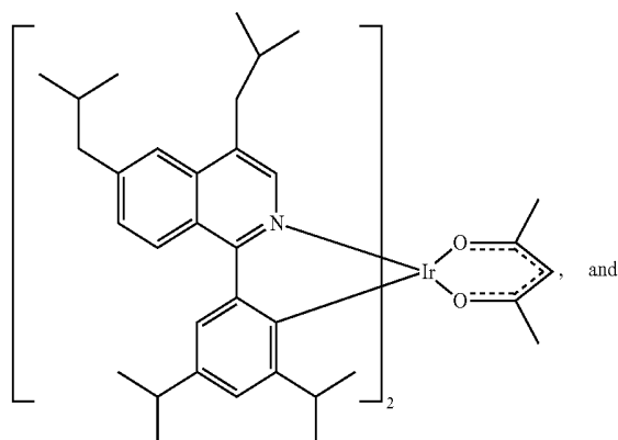
Compound 49
