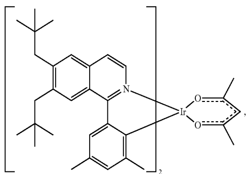
Compound 34
