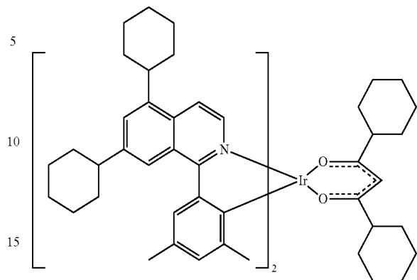
Compound 45
