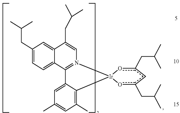
Compound 25
