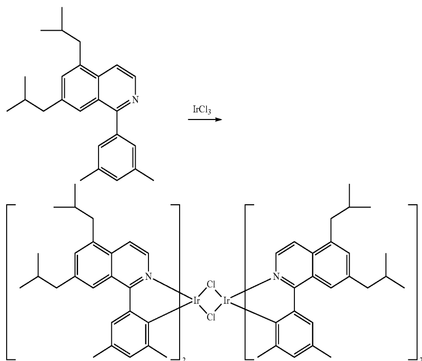
Synthesis of Iridium Dimer
