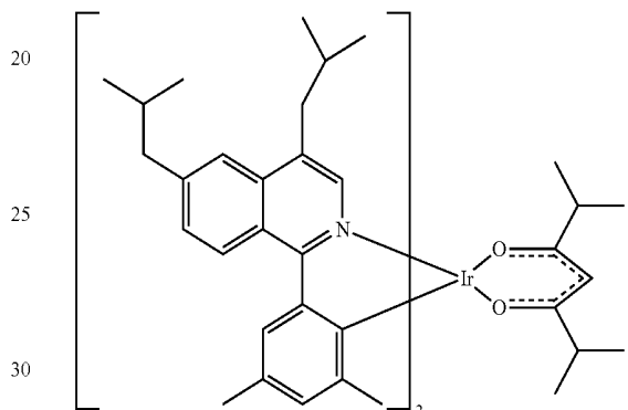
Compound 22
