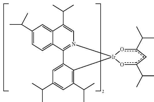
Compound 50
