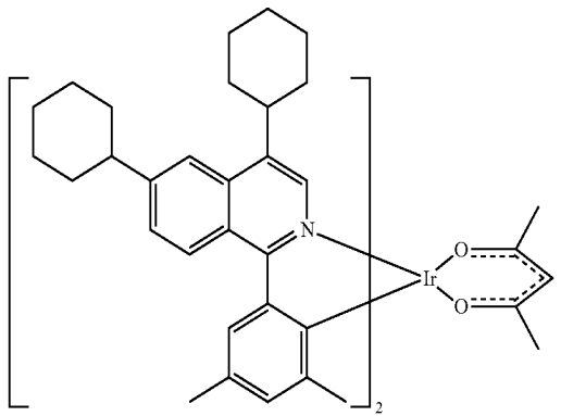
Compound 44
