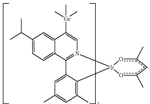
Compound 42
