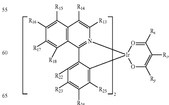
Formula IV
