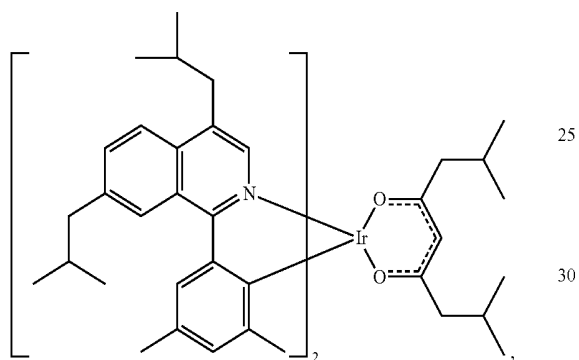
Compound 26
