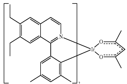
Compound 30
