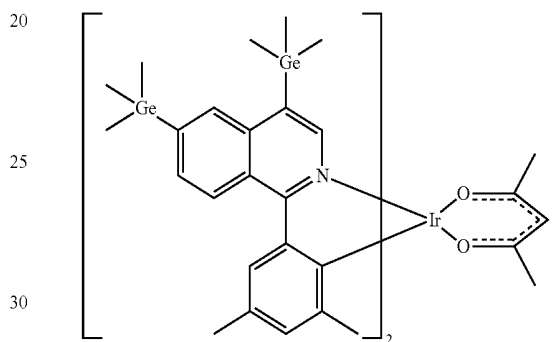
Compound 38
