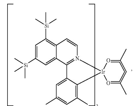
Compound 35
