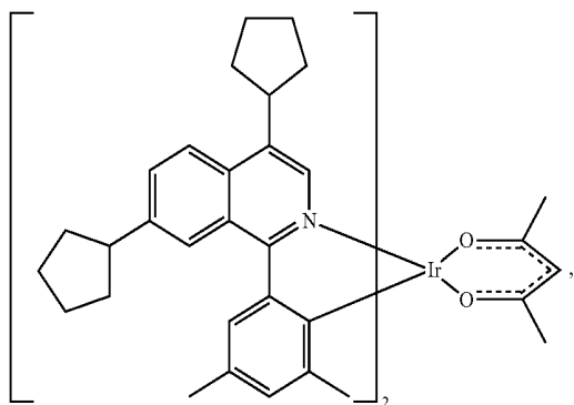
Compound 17
