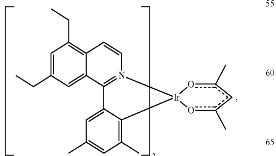
Compound 28
