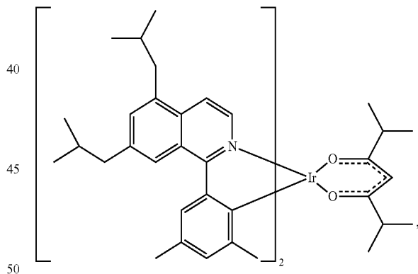
Compound 23
