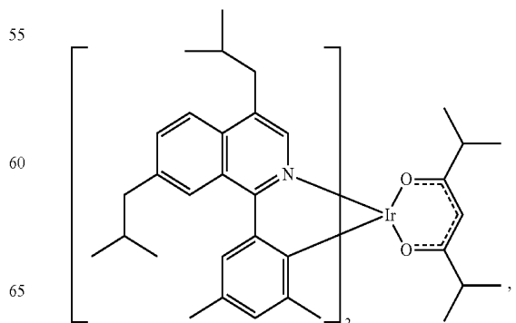
Compound 24
