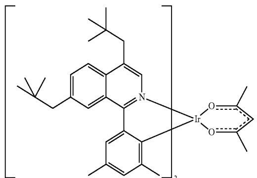
Compound 31
