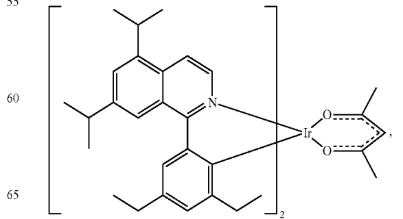
Compound 48
