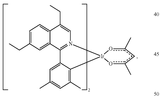
Compound 27
