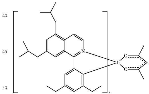
Compound 47
