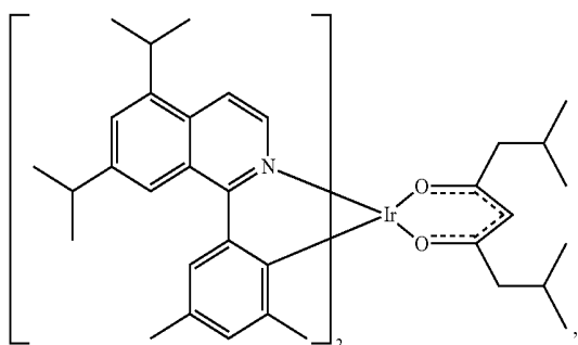
Compound 20
