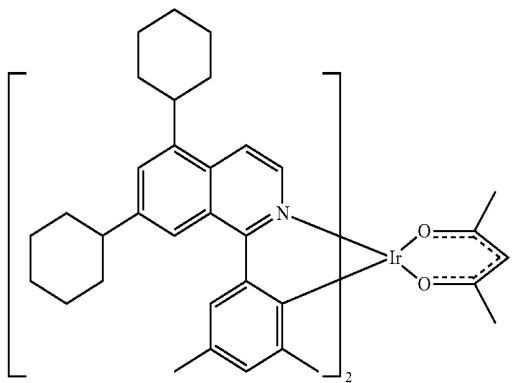
Compound 43
