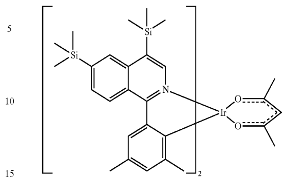
Compound 37
