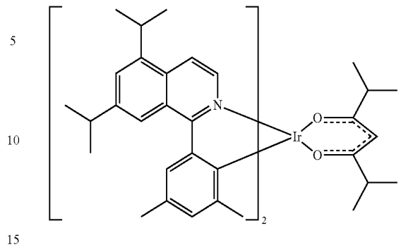
Compound 22
