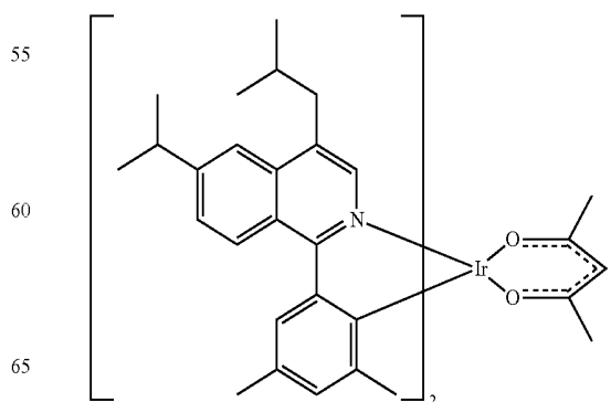
Compound 40
