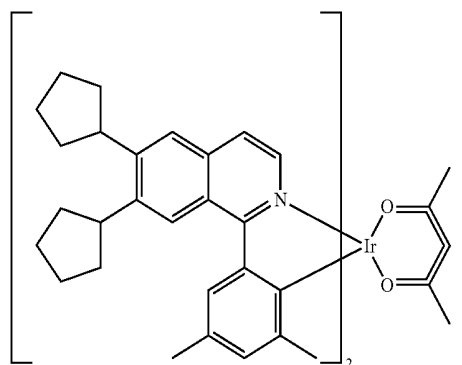
Compound 19
