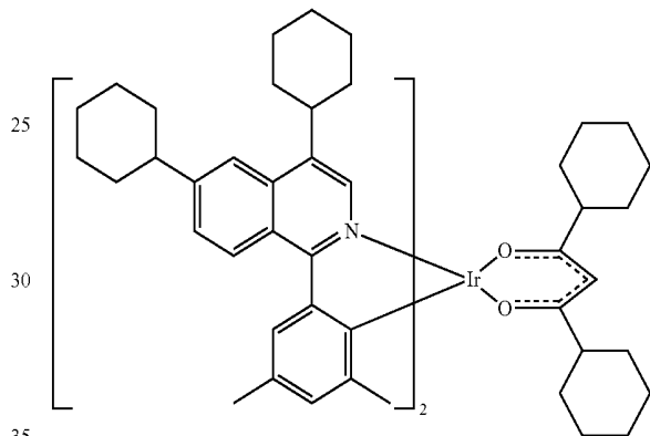
Compound 47
