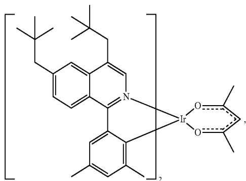
Compound 33
