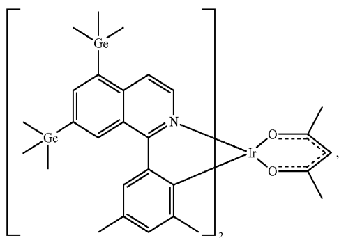
Compound 36
