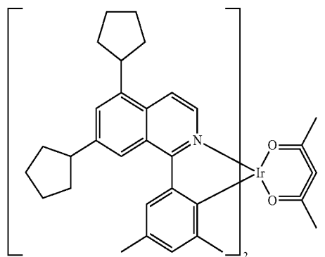
Compound 18
