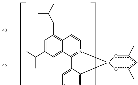
Compound 39
